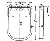
Figs. 1037-1038. Main Rod Guard, Atlantic (4-2) Locomotive. P. R. R.
